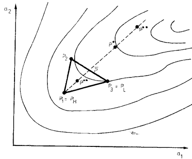
Fig. 4.8. The simplex method for function minimization
