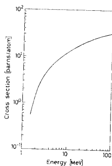
Fig. 2.25. Pair production cross section in lead
