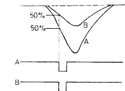
Fig. 17.4. Constant fraction discrimination
