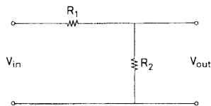
Fig. 14.25. Attenuator for slow signals (risetime > 100 ns)
