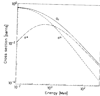
Fig. 2.23. Total Compton scattering cross sections
