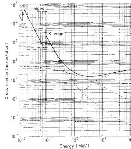
Fig. 2.29. Total photon absorption cross section for lead
