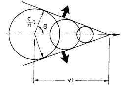
Fig. 2.9. Cherenkov radiation: an electromagnetic shock wave is formed when the particle travels faster than light in the medium.
