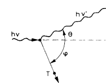
Fig. 2.22. Kinematics of Compton scattering
