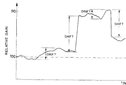
Fig. 8.21. PM gain drift and shift
