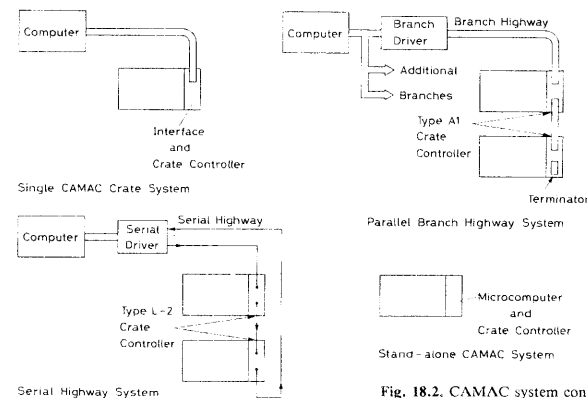
Fig. 18.2. CAMAC system configurations
