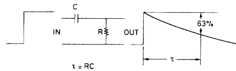
Fig. 14.30. CR high-pass filter or differentiating circuit
