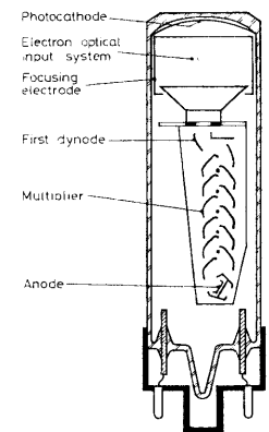
Fig. 8.1. Schematic diagram of a photomultiplier tube (from Schonkeren [9.1])
