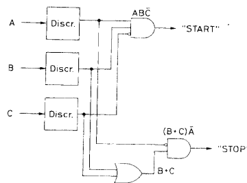
Fig. 16.9. Electronic logic for muon lifetime measurement
