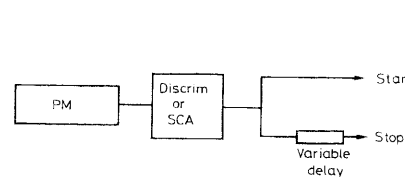
Fig. 17.13. Time scale calibration with a single source
