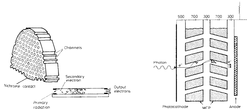
Fig. 8.6. Schematic diagram of a microchannel plate. The many channels act as continuous dynodes (from Dhawan [8.4]; picture © 1975 IEEE)
