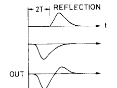
Fig. 14.29. Pulse clipping with reflection
