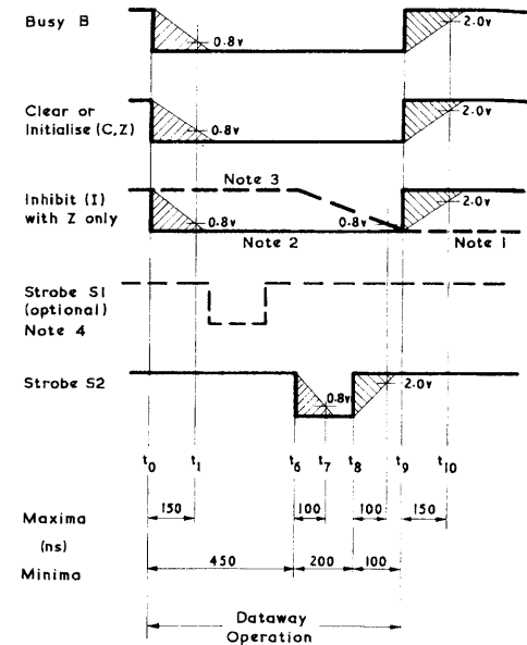
Fig. 18.5. Timing for unaddressed operations (from [18.2])
