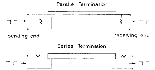
Fig. 13.7. Series and parallel termination
