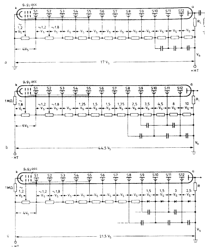
Fig. 8.10 a-c. Examples of PM voltage divider networks (after examples from Philips Catalog [8.7]): (a) divider network using positive high voltage; note the AC coupling capacitor at the anode, (b) a network using negative high voltage and decoupling capacitors for maintaining the voltages between the last few dynodes, (c) example of the use of Zener diodes to maintain voltages on the last few dynodes
