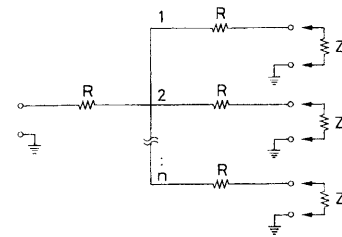
Fig. 14.27. Pulse splitter (or adder) for fast signals
