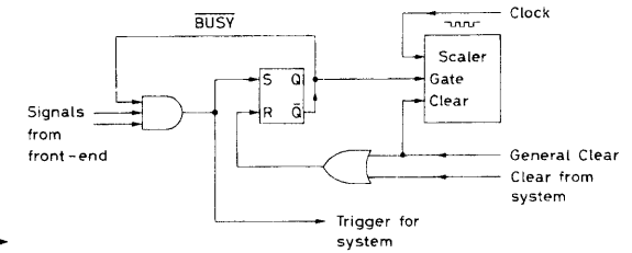
Fig. 16.4. INHIBIT or BUSY signal
