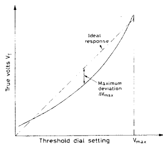
Fig. 14.16. Integral linearity of an SCA (after Milam [14.3])
