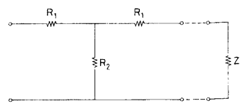
Fig. 14.26. Attenuator for fast pulses
