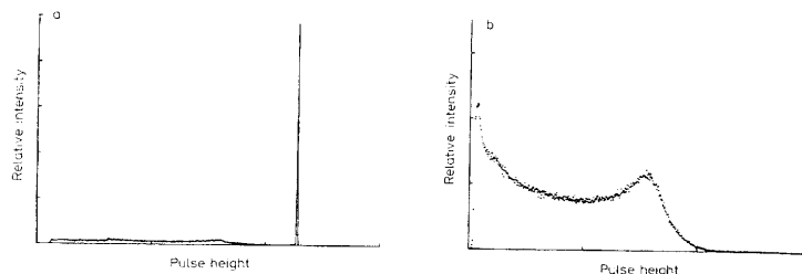
Fig. 5.2a, b. The response functions of two different detectors for 661 keV gamma rays. (a) shows the response of a germanium detector which has a large photoelectric cross section relative to the Compton scattering cross section at this energy. A large photopeak with a relatively small continuous Compton distribution is thus observed. (b) is the response of an organic scintillator detector. Since this material has a low atomic number Z , Compton scattering is predominant and only this distribution is seen in the response function
