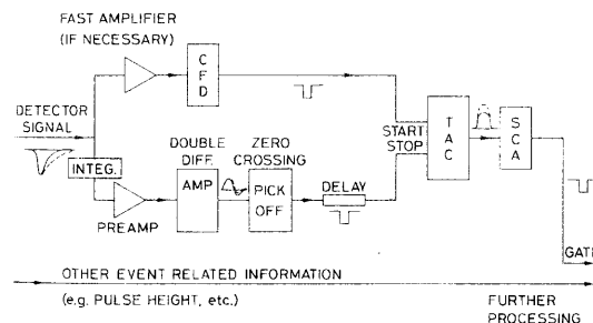
Fig. 15.15. A zero-crossing pulse shape discrimination circuit
