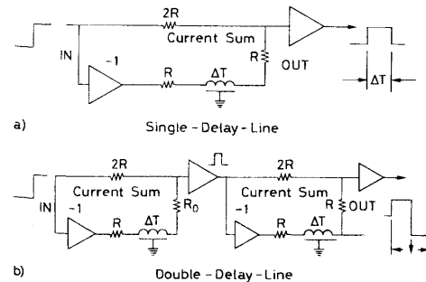
Fig. 14.10. (a) Single delay-line pulse shaping, (b) double delay line pulse shaping (from Ortec catalog [14.1])
