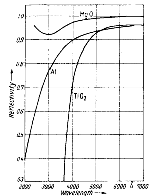
Fig. 9.3. Reflectivity of various materials (from Mott and Sutton [9.1])
