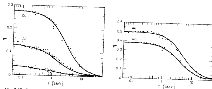
Fig. 2.17. Some measured electron backscattering coefficients for various materials. The electrons are perpendicularly incident on the surface of the sample (from Tabata et al. [2.24])
