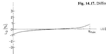
Fig. 14.17. Differential linearity of an SCA (after Milam [14.3])
