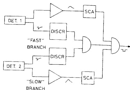
Fig. 15.14. A fast-slow coincidence system
