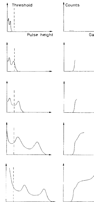
Fig. 9.19. Pulse height spectrum of ^{207}\text{Bi} observed with the detector in Fig. 9.16
