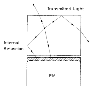
Fig. 9.1. Light collection in a typical scintillator
