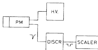
Fig. 9.17. Set-up for counter plateau measurement
