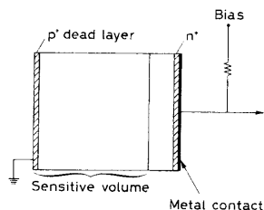
Fig. 10.8. Basic layout of a junction diode detector
