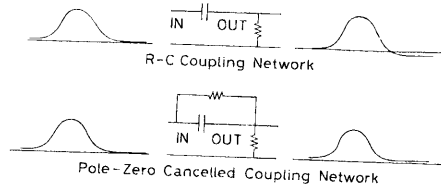
Fig. 14.7. Pole-zero cancellation circuit (from Ortec catalog [14.1])
