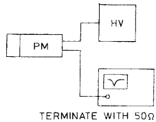
Fig. 9.15. Viewing the counter signal with an oscilloscope
