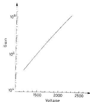
Fig. 9.23. Gain versus supply voltage on PM
