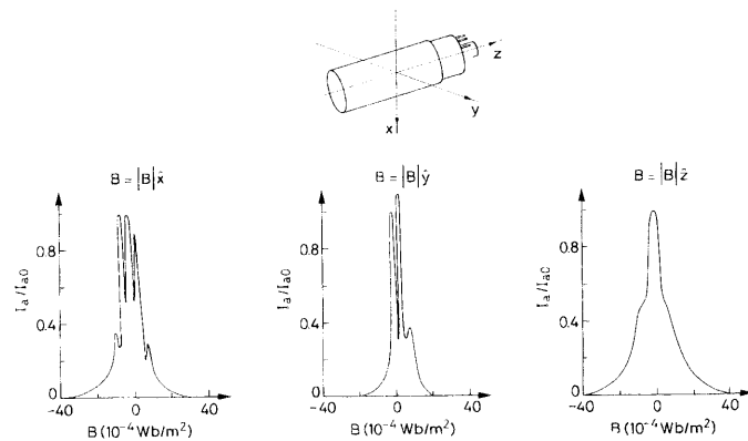
Fig. 8.17. Effect of magnetic fields on the anode current of an unshielded PM for different field orientations (from Schonkeren [8.1])
