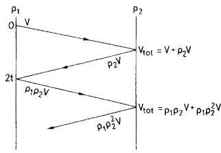
Fig. 13.5. Lattice diagram for multiple reflections
