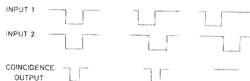
Fig. 15.9. Coincidence between pulses
