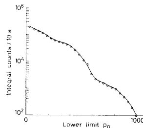
Fig. 9.21. Integral counting curve for ^{207}\text{Bi}
