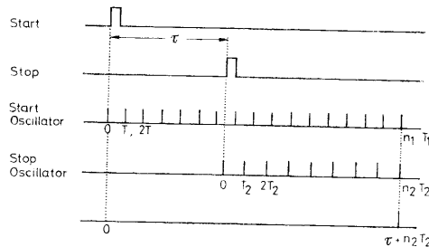
Fig. 17.11. Working principle of the vernier TDC
