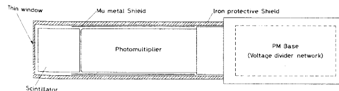
Fig. 7.1. Schematic diagram of a scintillation counter
