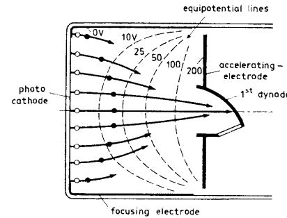
Fig. 8.14. Transit time difference (from Schonkeren (8.1))
