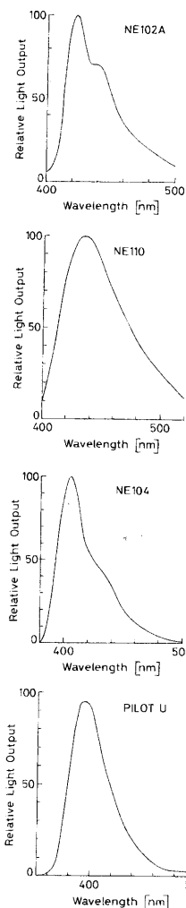
Fig. 7.5. Light emission spectra for several different plastic scintillators (from Nuclear Enterprises catalog [7.1])
