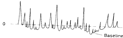
Fig. 14.8. Baseline shift at high count rates
