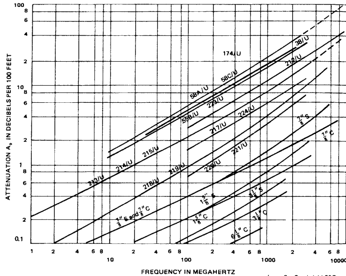
Fig. 13.8. Attenuation constants for various cables
