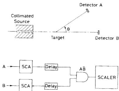
Fig. 16.6. Simple set-up for Rutherford scattering
