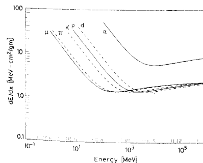
Fig. 2.4. The stopping power dE/dx as function of energy for different particles
