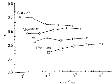
Fig. 2.27. Values of the parameter b in (2.129) for various materials (from [2.15]).
