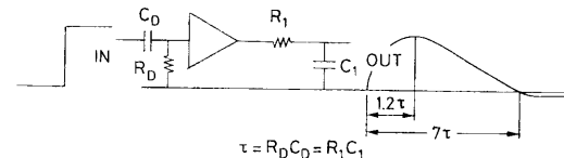
Fig. 14.5. CR-RC pulse shaping network. Because of residual differentiations in the preamplifier, the width and cross-over point of the resultant signal are not those calculated theoretically (from Ortec catalog [14.1])
