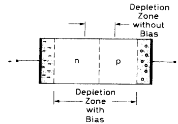
Fig. 10.7. Reversed-bias junction
