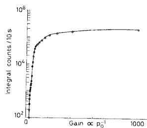
Fig. 9.22. Integral counting curve vs. gain (arbitrary units)
