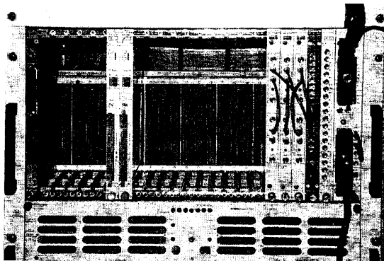
Fig. 18.1. A CAMAC crate and modules
