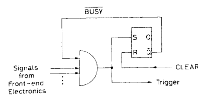
Fig. 16.4. INHIBIT or BUSY signal
