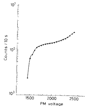
Fig. 9.18. Measured plateau curve for plastic scintillator detector shown in Fig. 9.16 using a ^{207}\text{Bi} source
