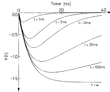
Fig. 8.13. Output signals for various time constants \tau (after Wright (8.8))
