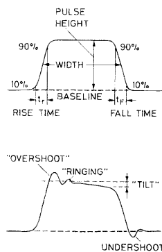
Fig. 11.1. Pulse signal terminology
