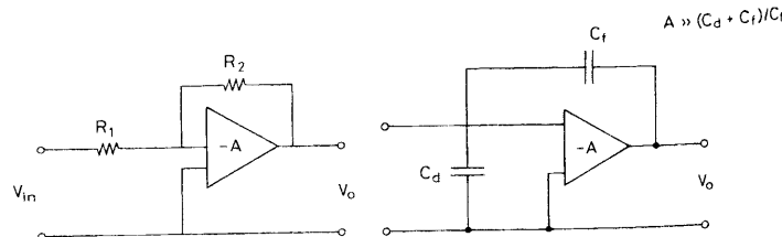
Fig. 14.1. Schematic diagram of a voltage-sensitive preamplifier
