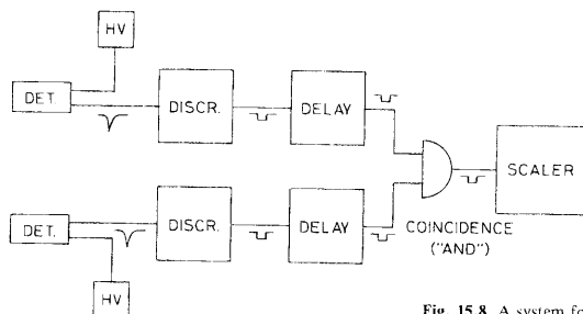
Fig. 15.8. A system for coincidence measurement
