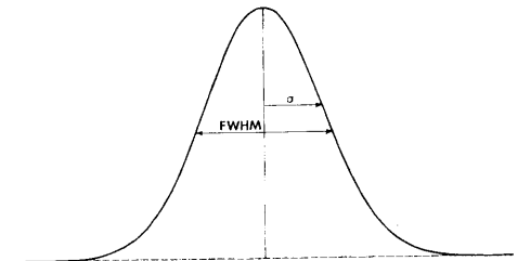
Fig. 4.4. Relation between the standard deviation \sigma and the full width at half-maximum (FWHM)
