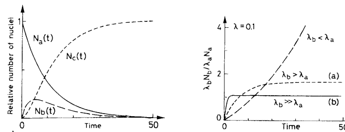
Fig. 1.7. Radioactive decay of a three nucleus chain
