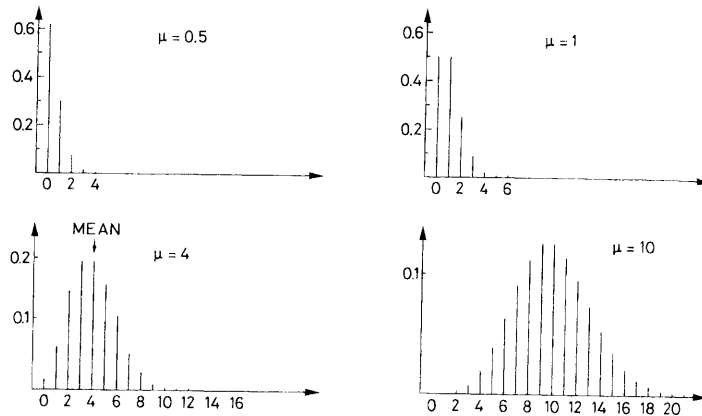
Fig. 4.2. Poisson distribution for various values of \mu
