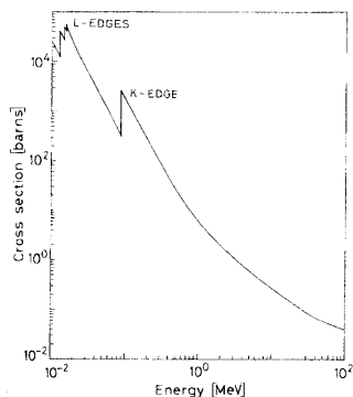
Fig. 2.21. Calculated photoelectric cross section for lead
