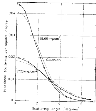
Fig. 2.15. Angular distribution of 15.7 MeV electrons scattered from a thin Au foil (from Hanson et al. [2.23]). The experimental values are compared with the Gaussian approximation to multiple scattering
