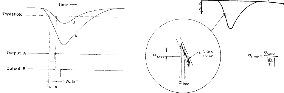
▲ Fig. 17.1. Walk in a discriminator or SCA. Coincident signals with different amplitudes cross the threshold at different times. An additional walk effect occurs because of the finite charge which must be integrated on a capacitor to trigger the discriminator or SCA.
