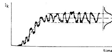
Fig. 8.16. Statistical noise from a PM (from Philips Catalog [8.7])
